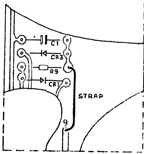
MODIFICATION SMD CARD
